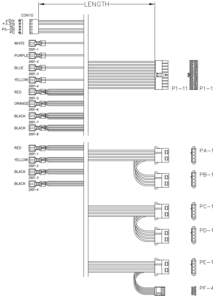
FIG-1:DC OUTPUT CONNECTOR
