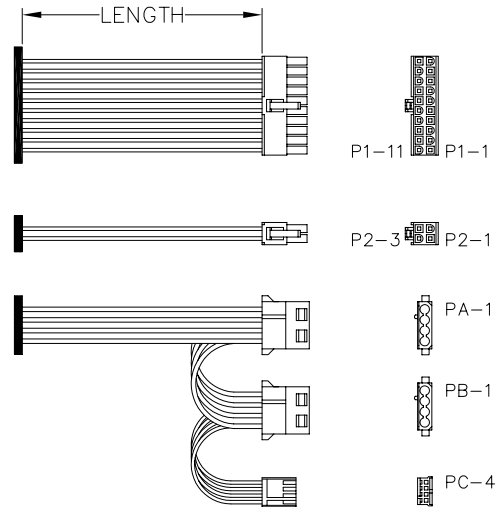
FIG-1:DC OUTPUT CONNECTOR
