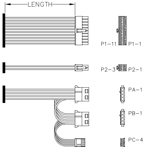
FIG-1: DC OUTPUT CONNECTOR
