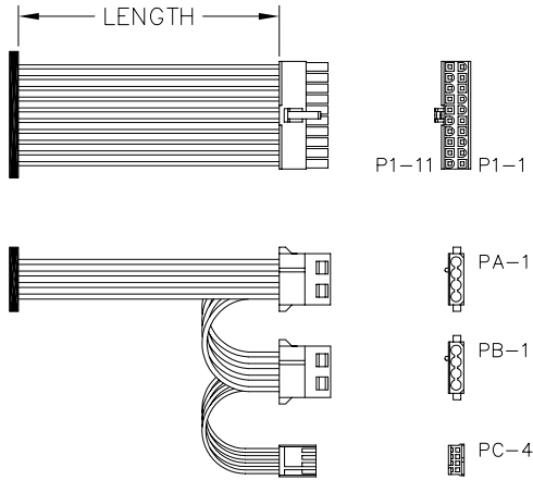
FIG-1: DC OUTPUT CONNECTOR
