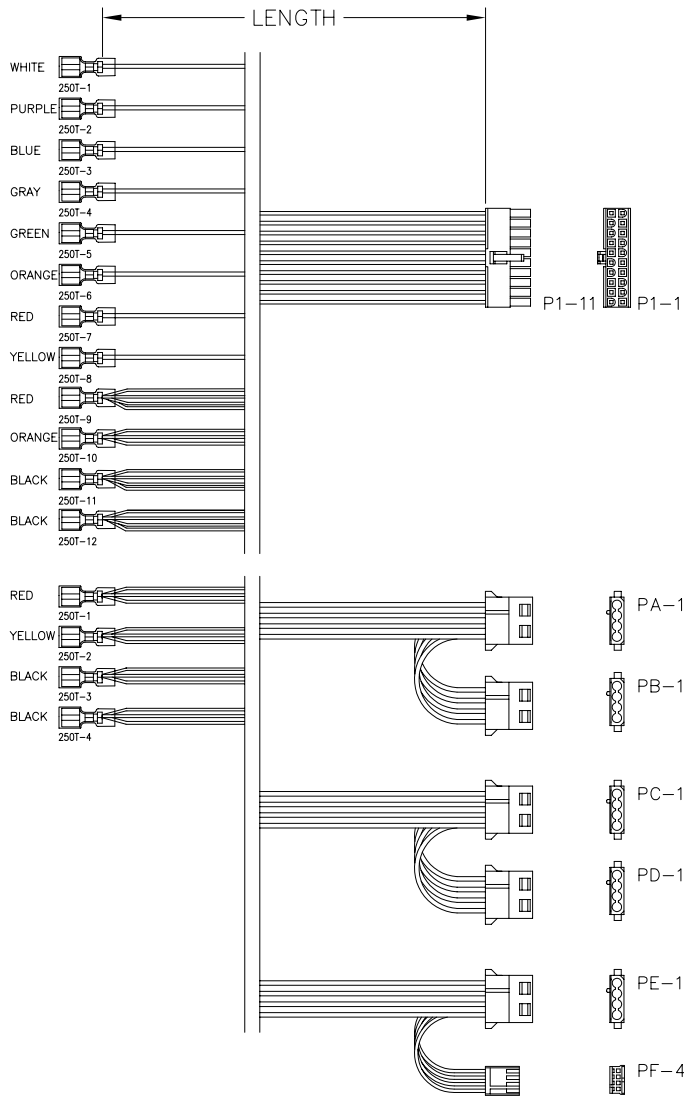
FIG-1:DC OUTPUT CONNECTOR
